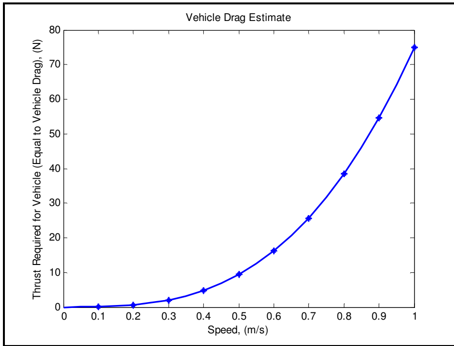
Figure 4-1: Required thrust estimate for a low-speed, high-drag AUV.
