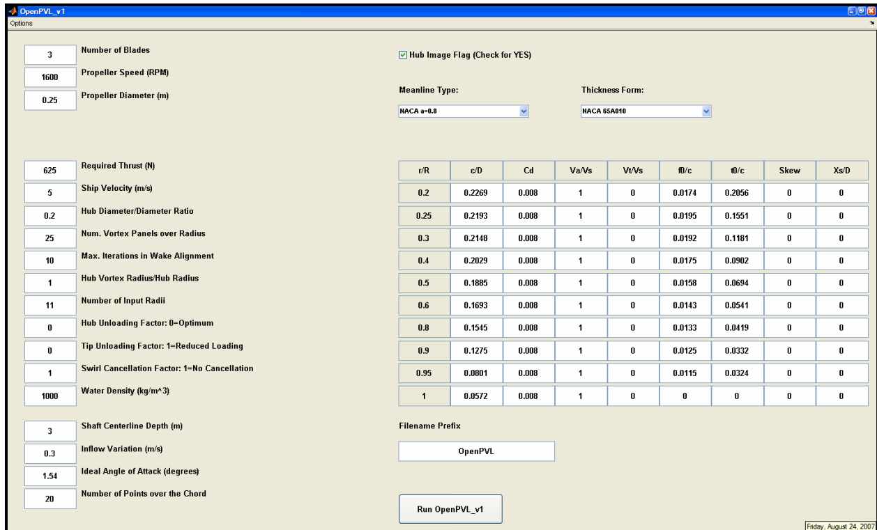
Figure 2-5: Single Propeller Design GUI.
