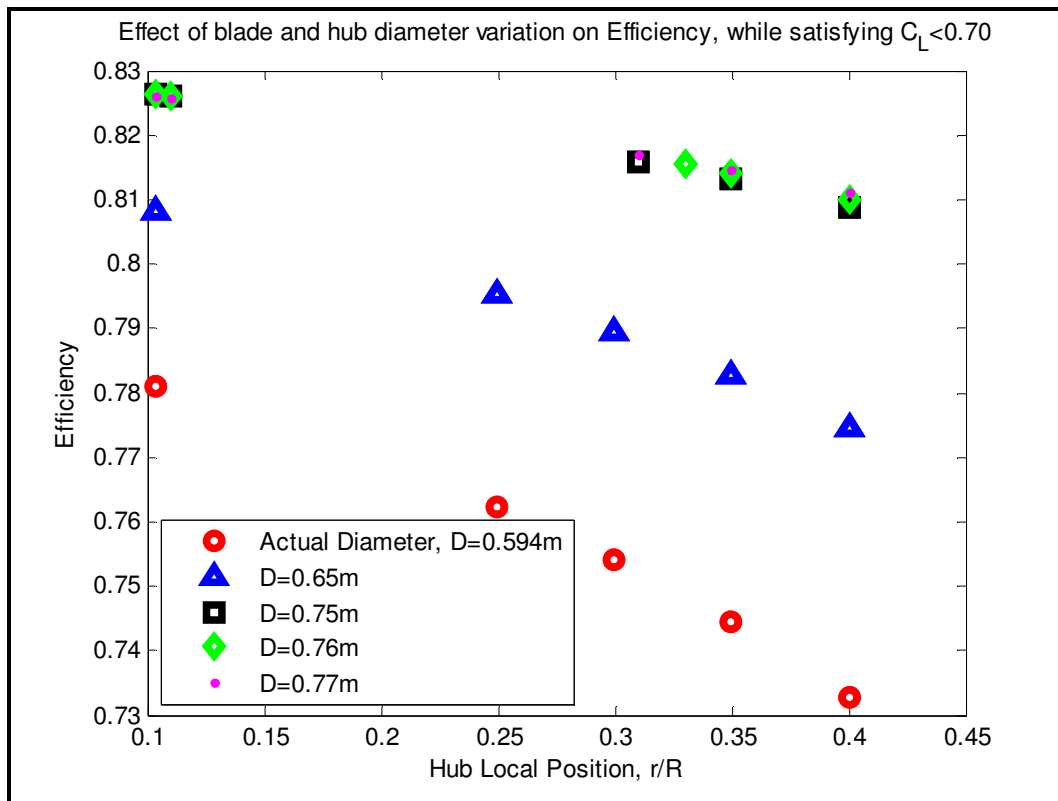
Figure 5-3: Efficiency vs. variation of blade hubs for different diameters of the off-the-shelf propeller. In this case, C_L < 0.7 is satisfied for D = 0.76\text{m} and 0.77\text{m} .
